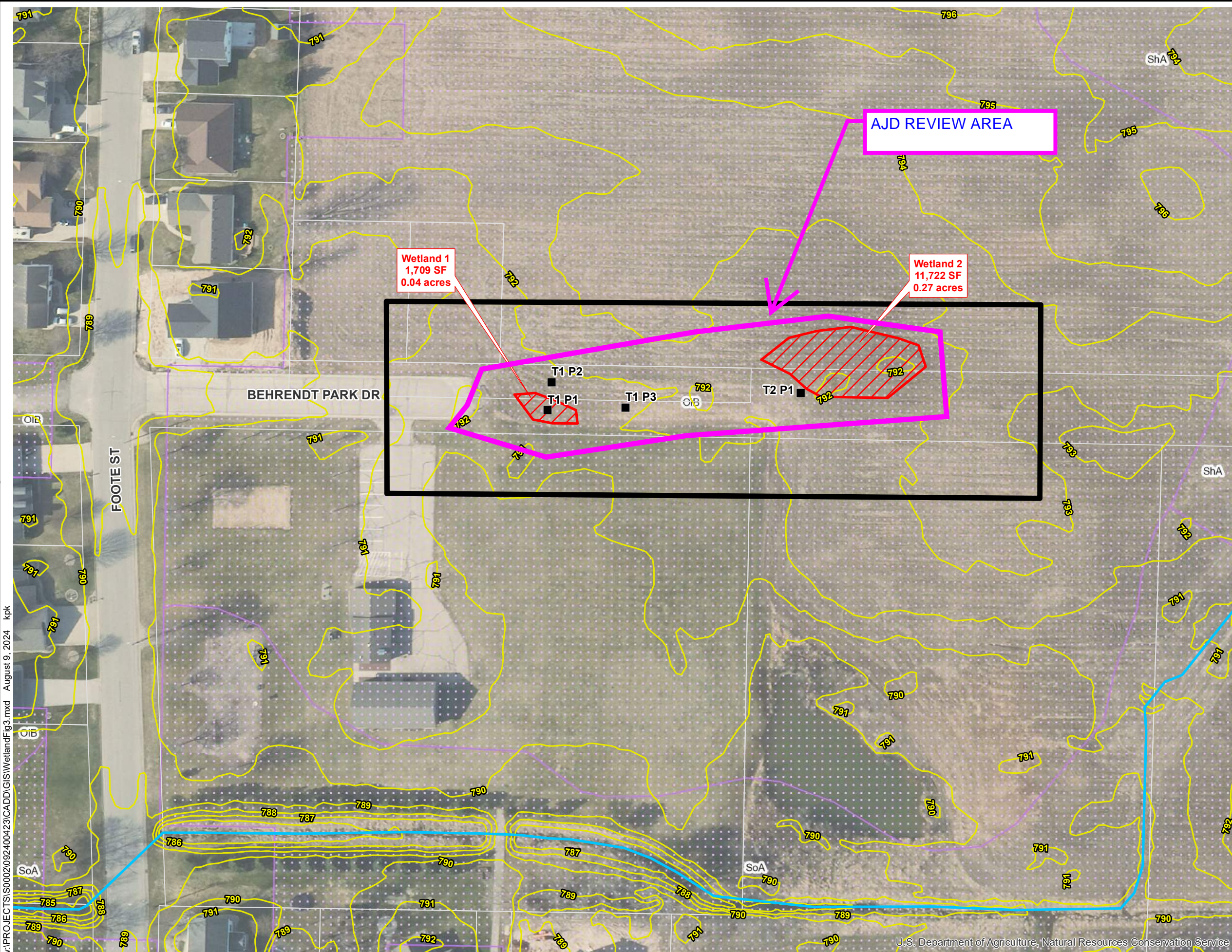
FIGURE 3 WETLAND DELINEATION MAP MAINLINE DRIVE EXTENSION CITY OF SEYMOUR OUTAGAMIE COUNTY, WISCONSIN
