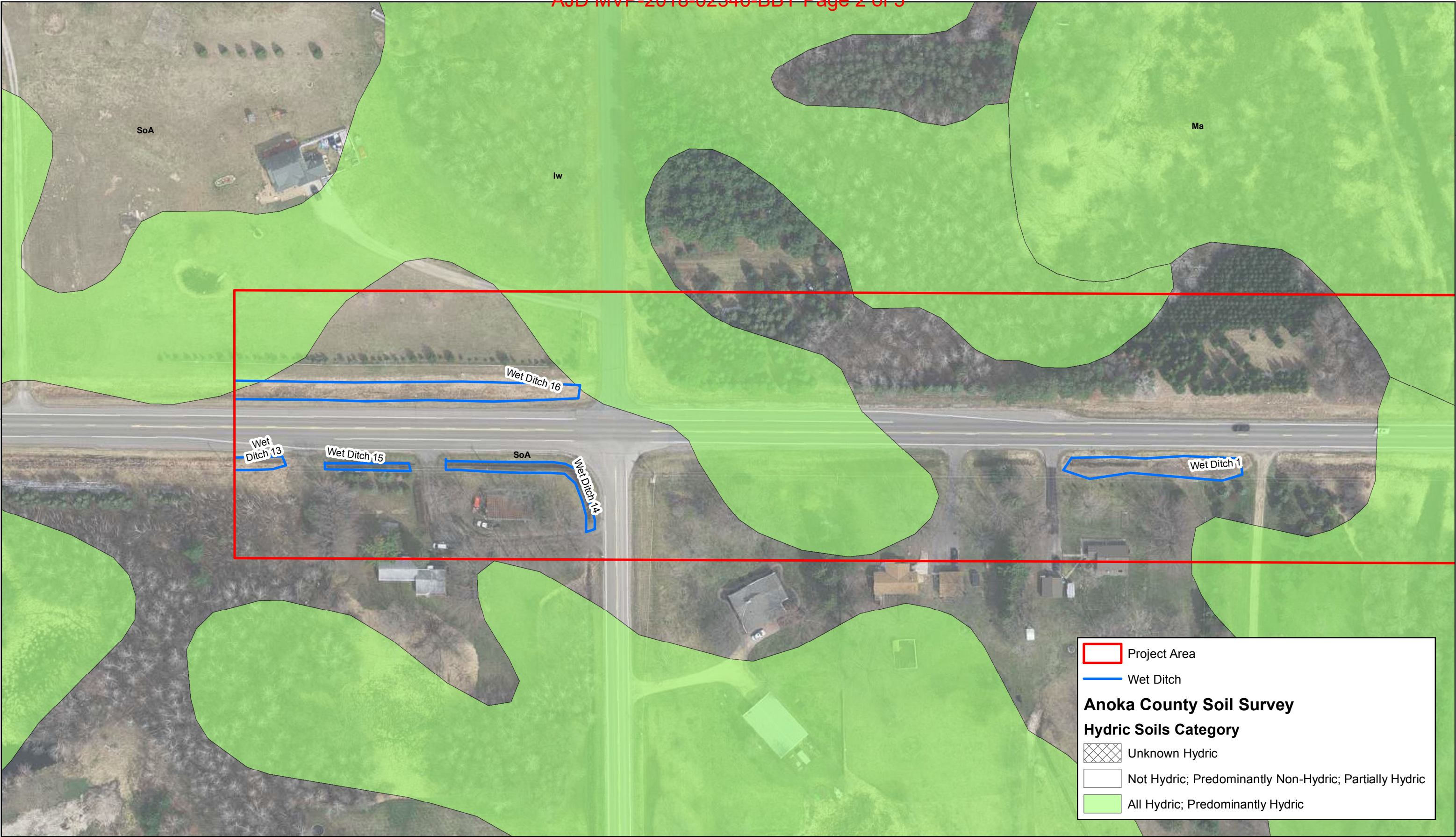
Figure 7b - Wet Ditches CSAH 18 Anoka County
