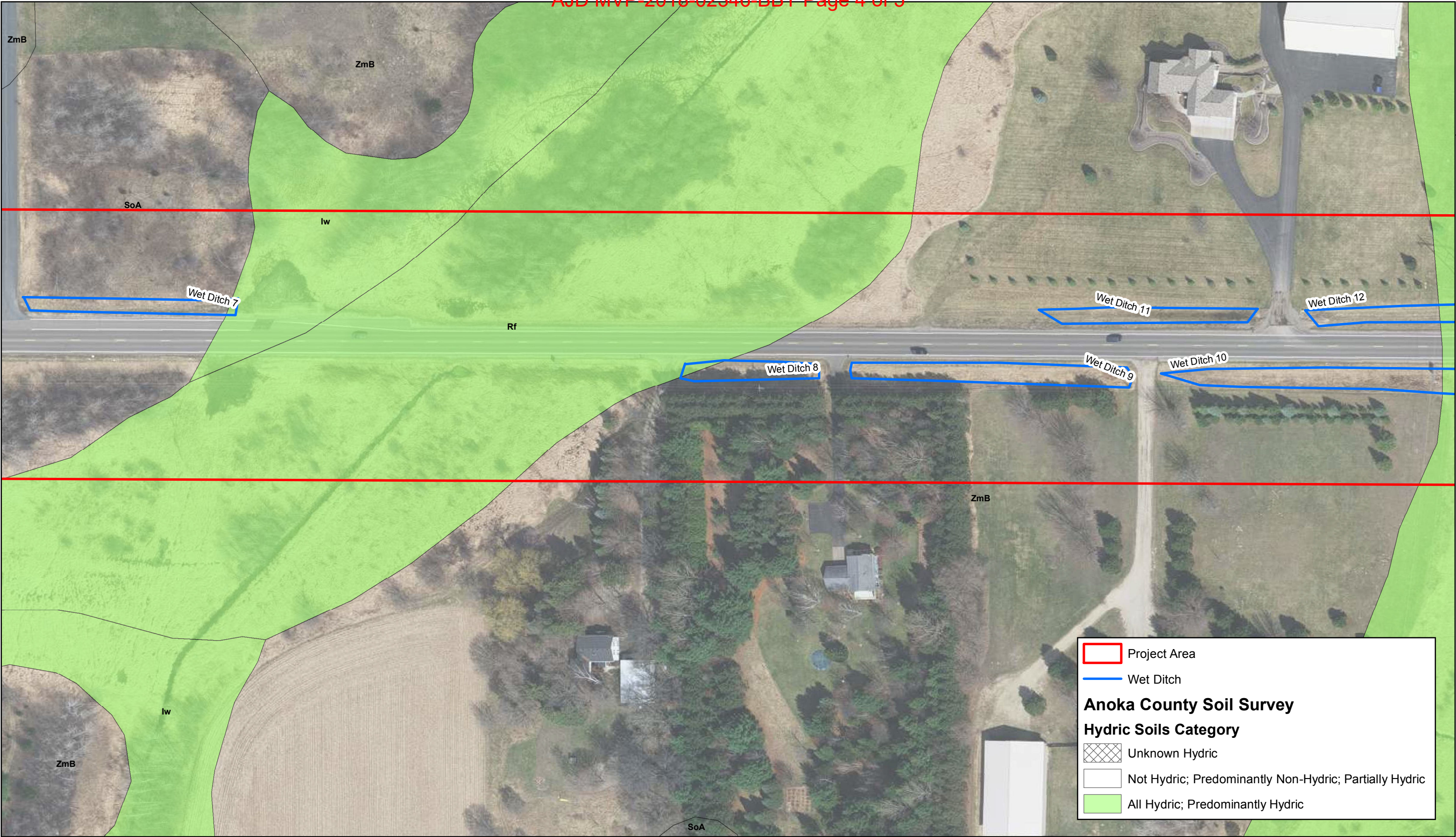
Figure 7d - Wet Ditches CSAH 18 Anoka County
