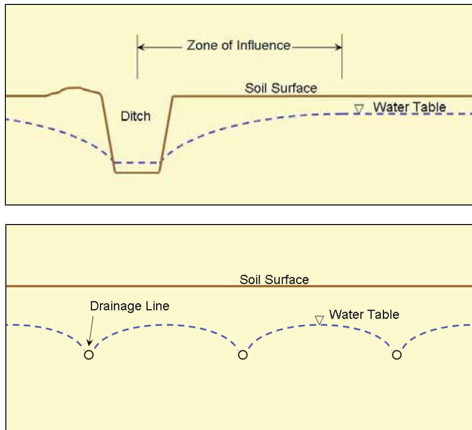
Figure 47. Effects of ditches (upper) and parallel subsurface drainage lines (lower) on the water table.
