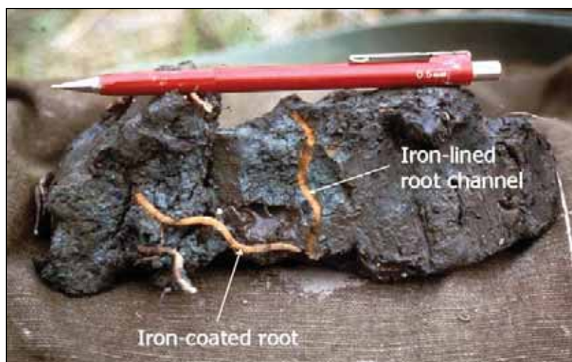
Figure 40. Iron-oxide plaque (orange coating) on a living root. Iron also coats the channel or pore from which the root was removed.
