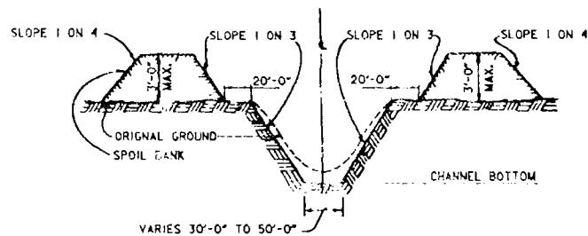
TYPICAL SECTION (MUSTINKA RIVER)
