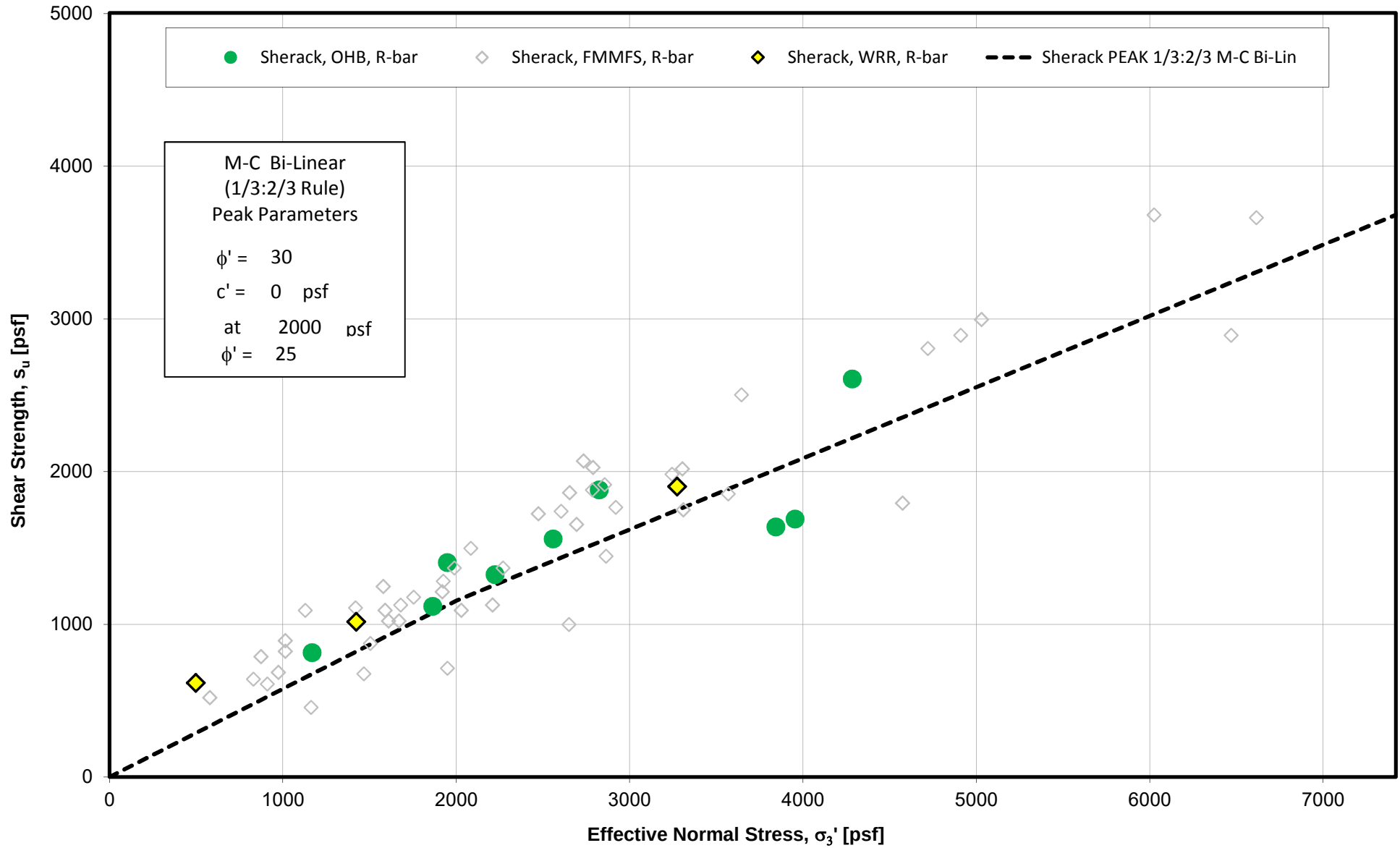
Figure 3 Sherack Drained Shear Strength @ Peak Stress Mohr-Coulomb Effective Stress Plot
