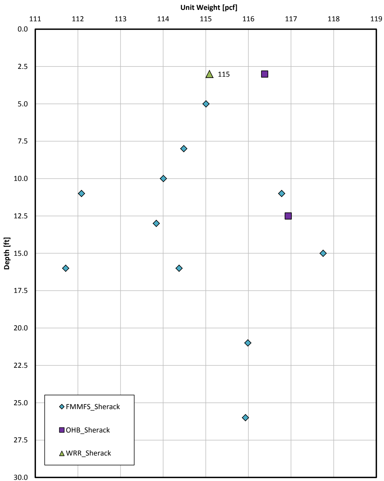
Figure 10 Sherack Unit Weights 100% Compaction Based on Standard Proctor Results
