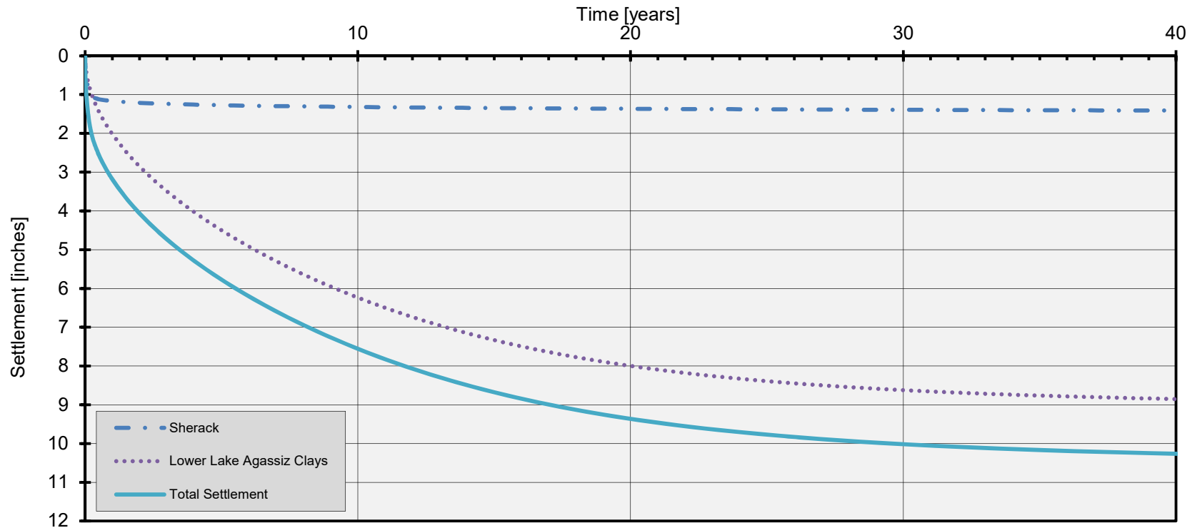
Total Settlement vs Time Due to Embankment Construction
