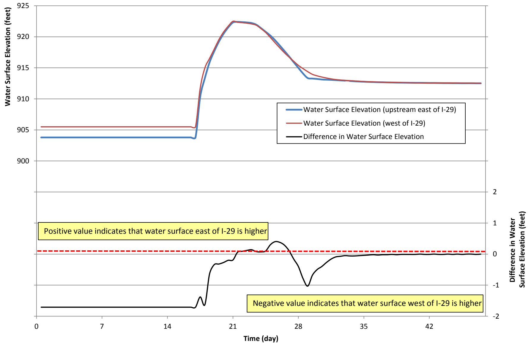
Figure 4. Difference in Pool Elevation East and West of I-29 during the 100-Year Event
