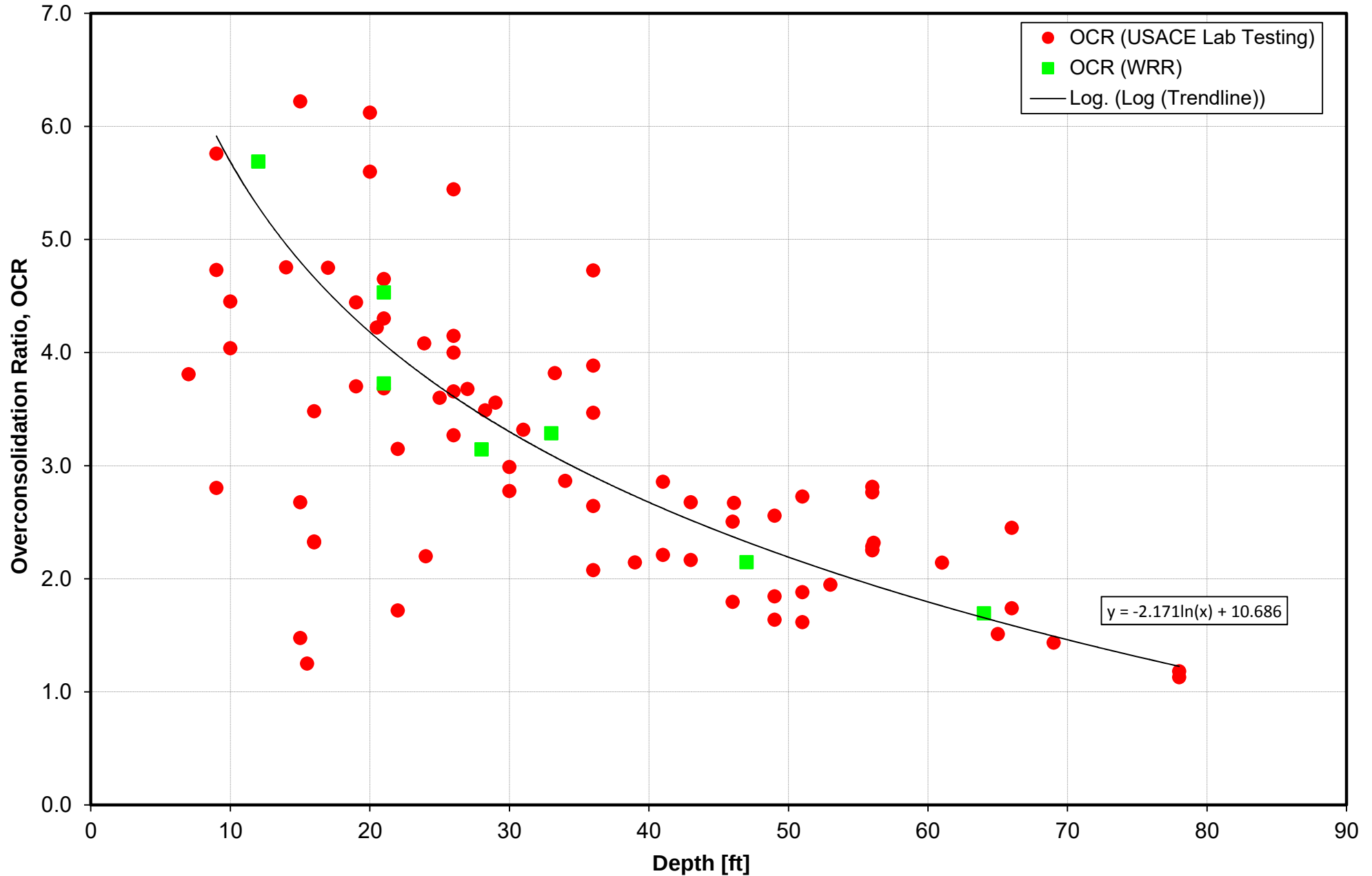
FIGURE 11 Overconsolidation Ratio vs Depth Fargo-Moorhead Metropolitan Feasibility Study
