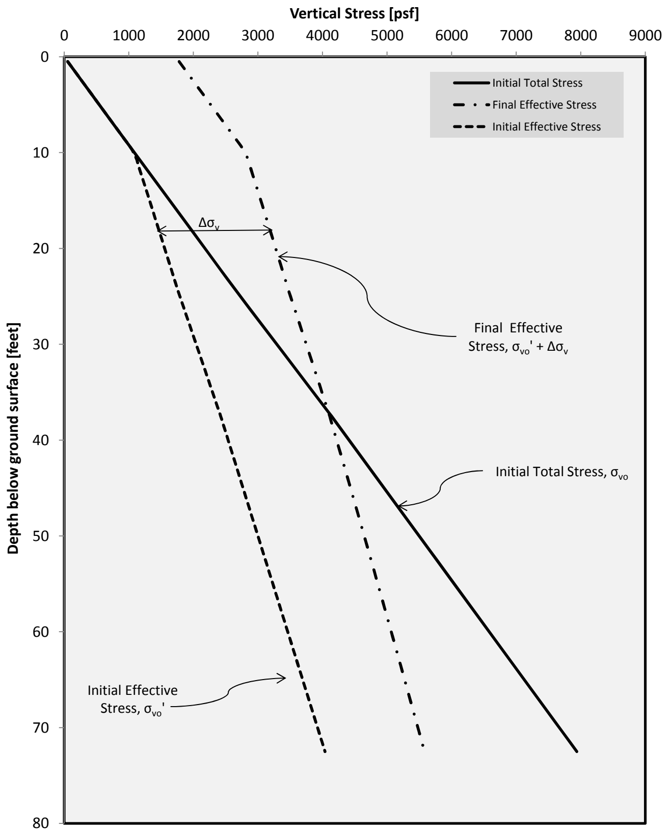
FIGURE 1 Stress History and Stress Change Profile
