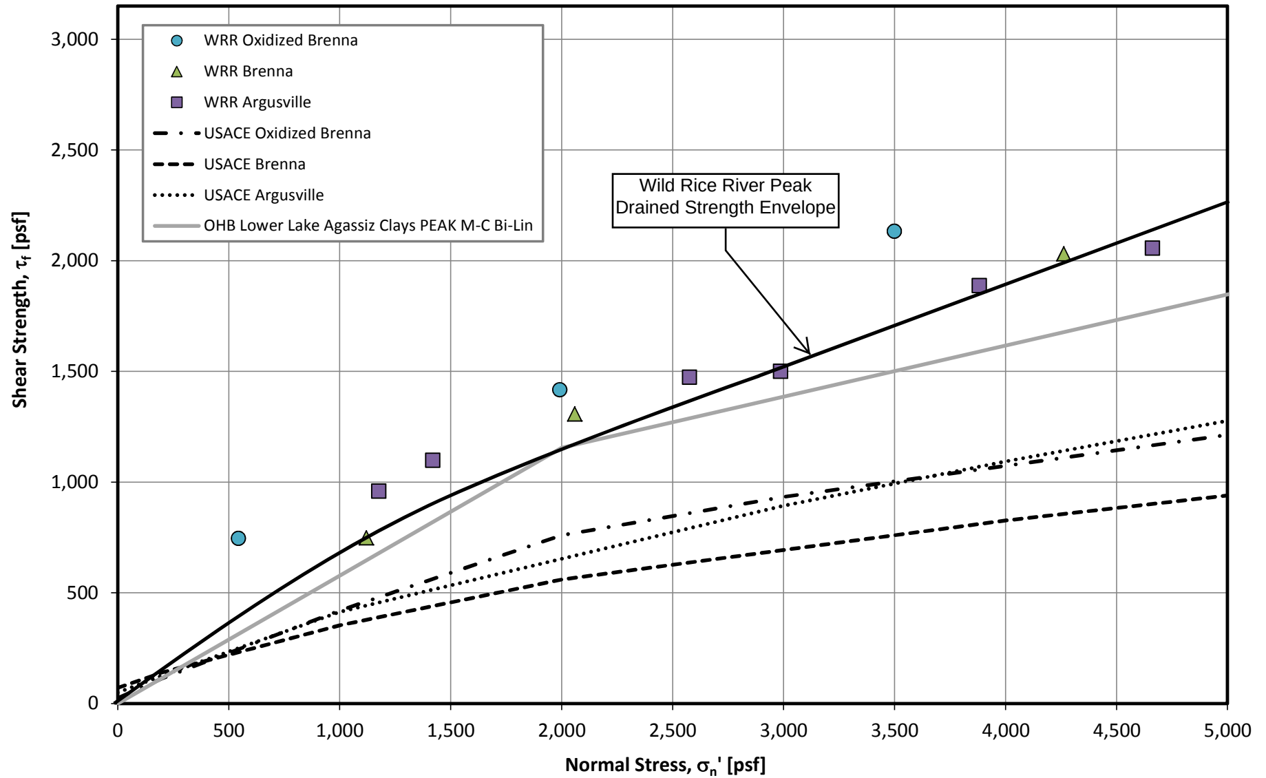
FIGURE 7 Oxidized Brenna, Brenna, and Argusville Drained Peak Shear Strength Mohr-Coulomb Effective Stress Plot
