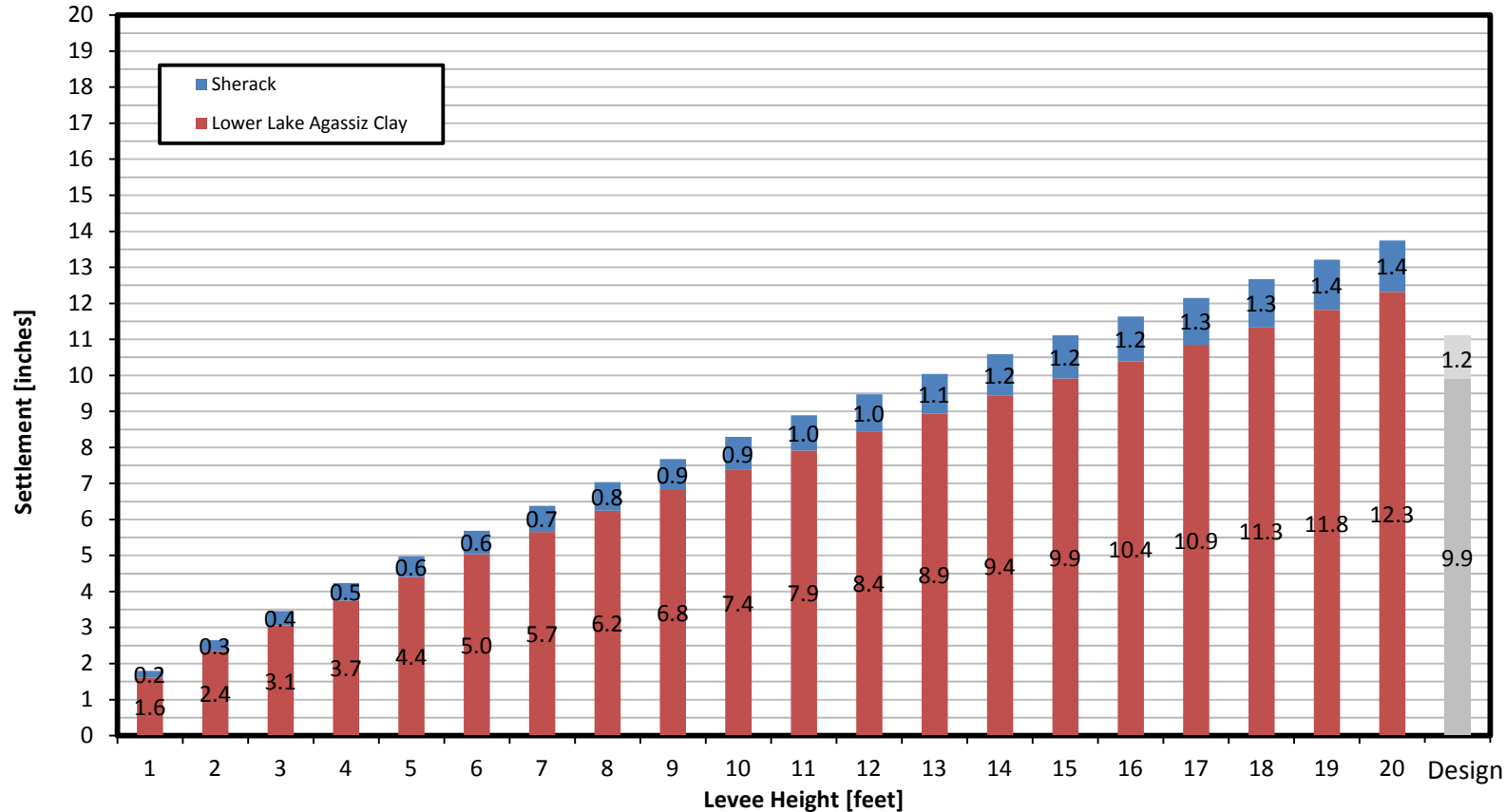
Wild Rice River Primary and Secondary Compression per Geologic Unit
