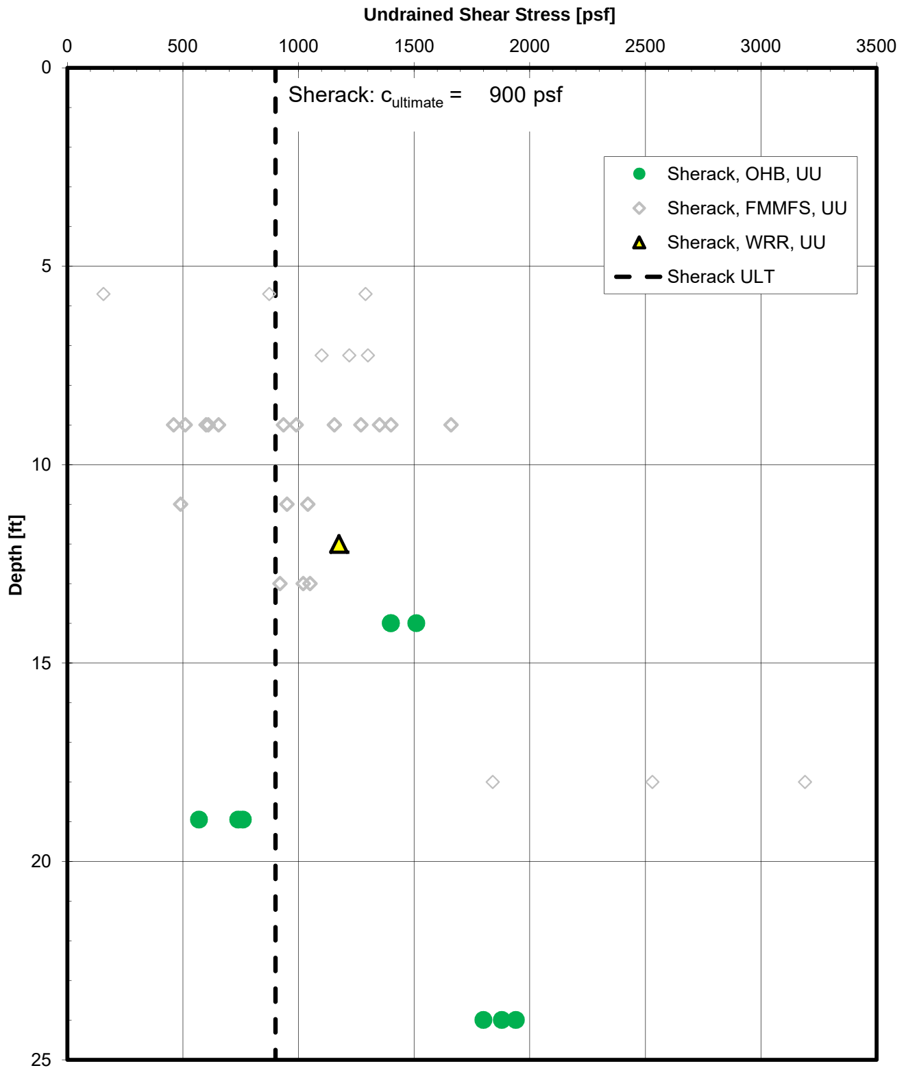
Figure 4 Sherack Formation Undrained Shear Strength (UU) Data @ 15% Strain
