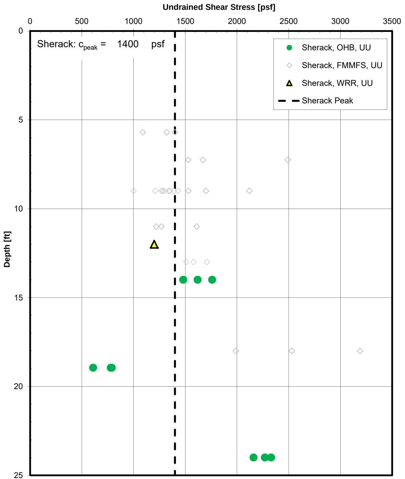
Figure 5 Sherack Formation Peak Undrained Shear Strength (UU) Data
