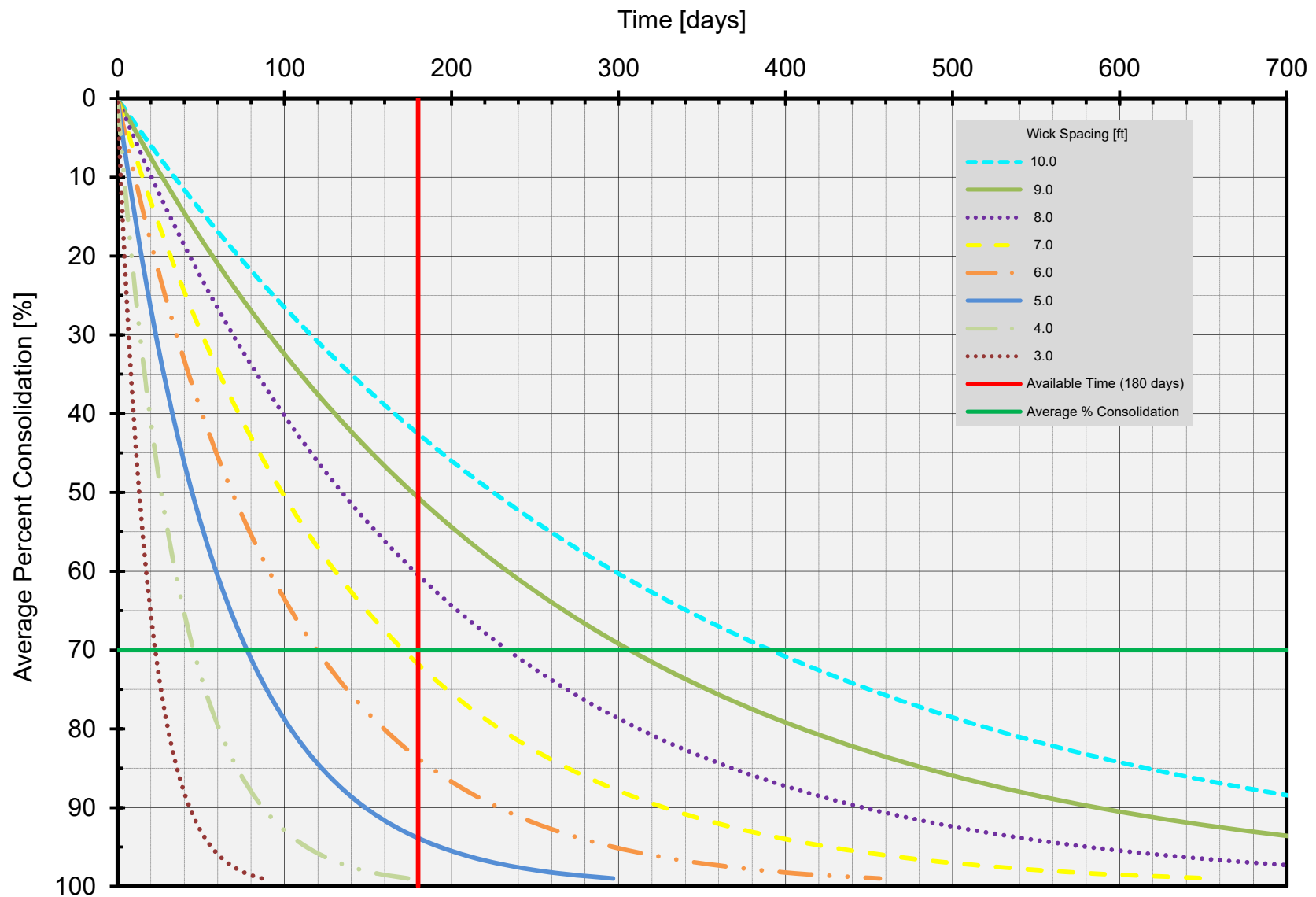
FIGURE 2 Time versus Consolidation Due to 11 Feet of Surcharge Load and Wick Drains Embankment 7 - 15 feet
