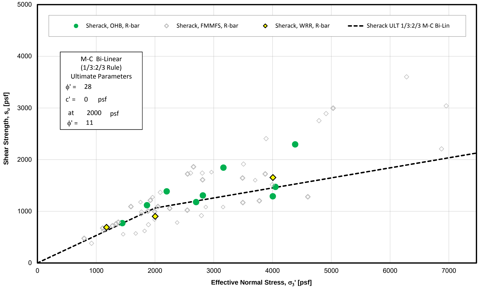
Figure 2 Sherack Drained Shear Strength @ 15% Strain Mohr-Coulomb Effective Stress Plot
