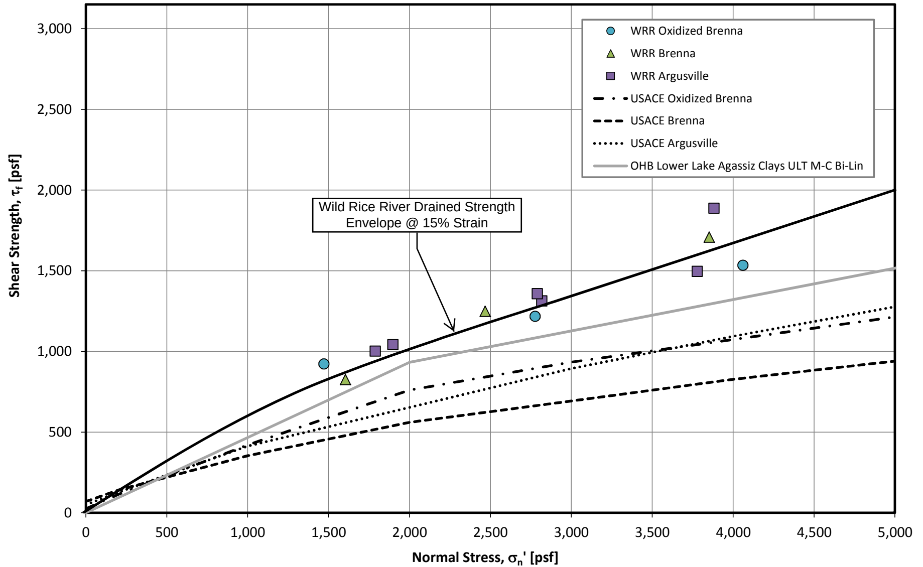
FIGURE 6 Oxidized Brenna, Brenna, and Argusville Drained Shear Strength @15% Strain Mohr-Coulomb Effective Stress Plot
