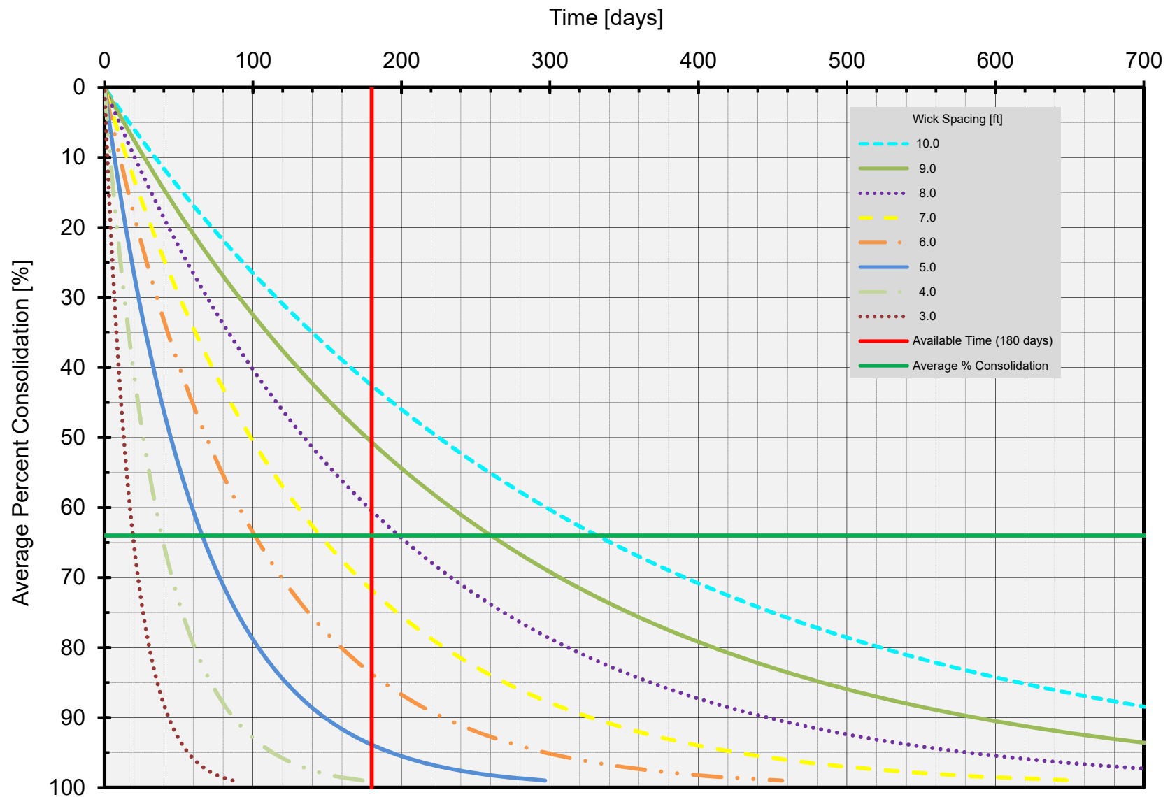
FIGURE 3 Time versus Consolidation Due to 6 Feet of Surcharge Load and Wick Drains Embankment 0 - 7 feet
