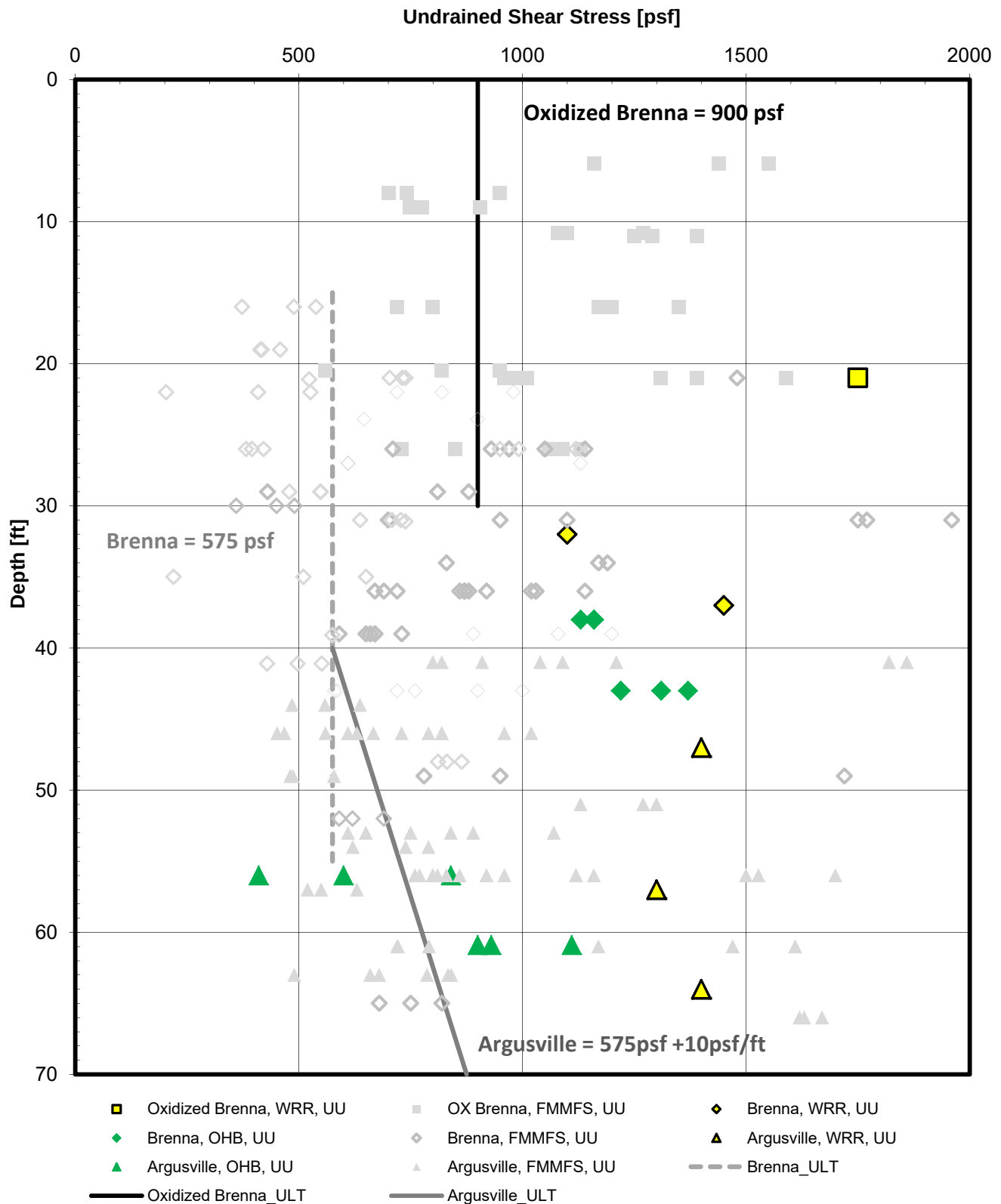
Figure 8 Oxidized Brenna, Brenna, and Argusville Undrained Shear Strength (UU) Data @ 15% Strain
