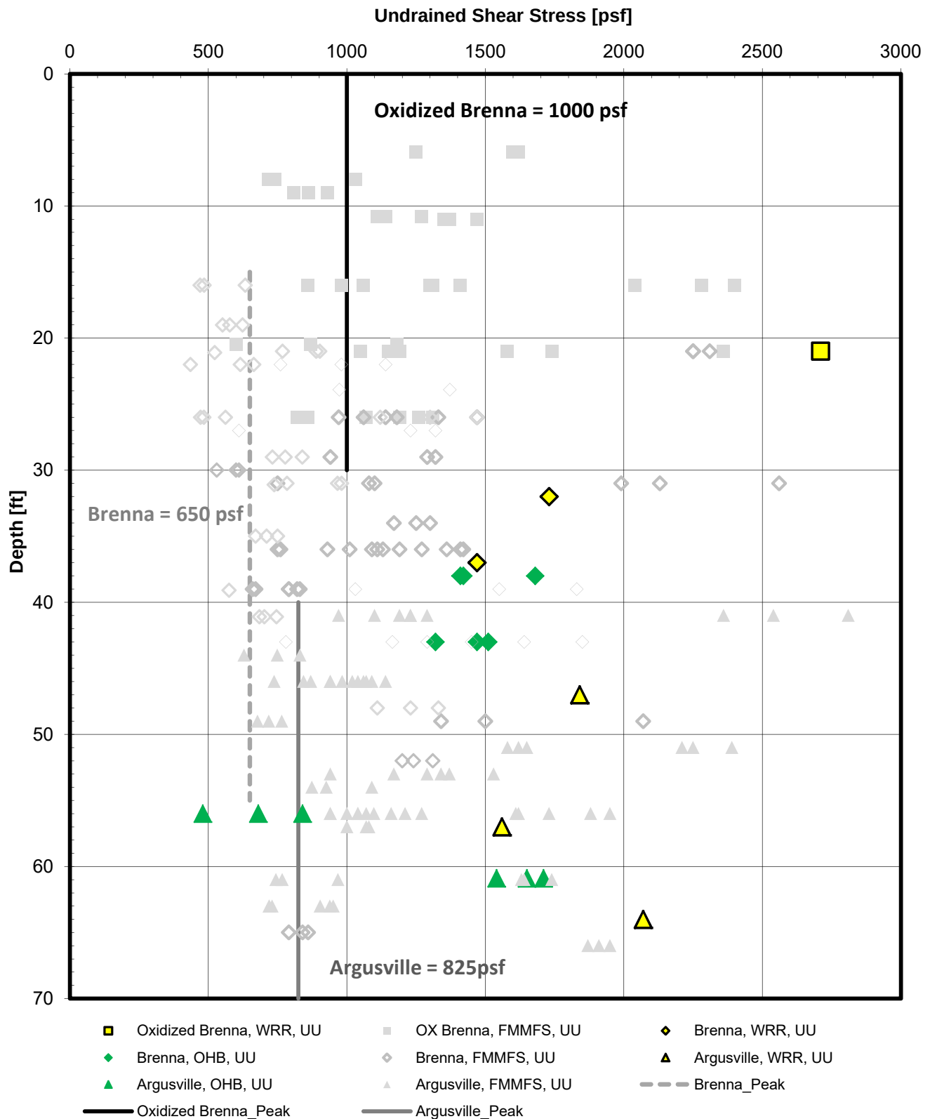
Figure 9 Oxidized Brenna, Brenna, and Argusville Peak Undrained Shear Strength (UU) Data
