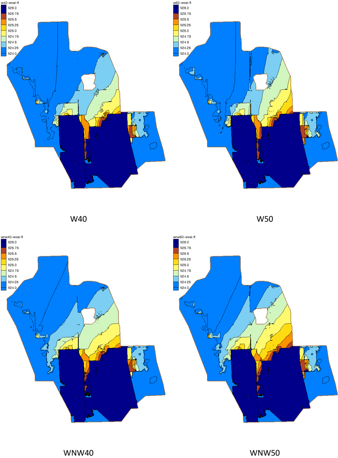
Figure 21: Water surface elevation with wind setup for winds from the west and west-northwest
