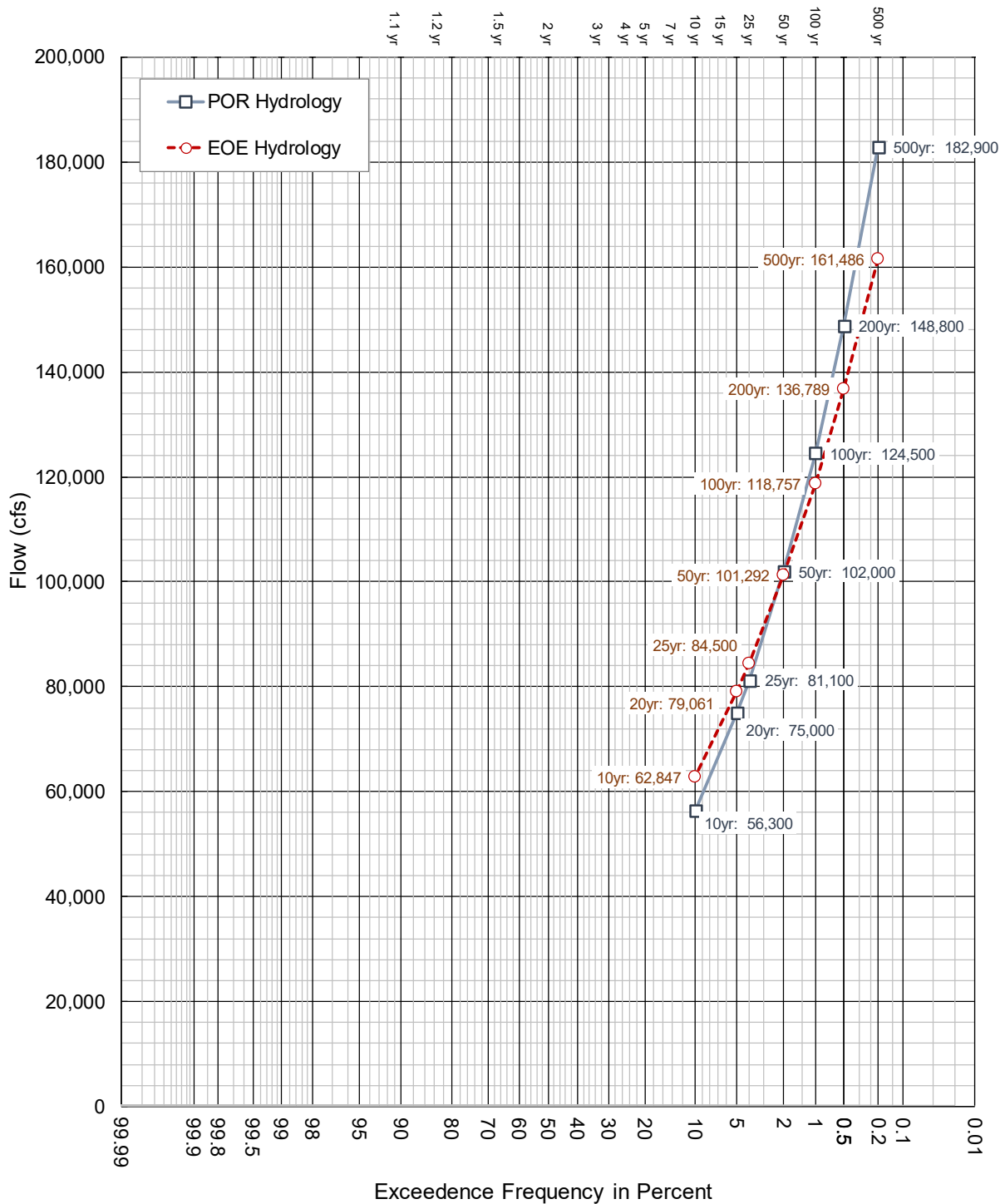
Exhibit 8 - Discharge Frequency Curve at Drayton Gage Period of Record (POR) Hydrology vs Expert Opinion Elicitation / Wet Cycle (EOE/WET) Hydrology
