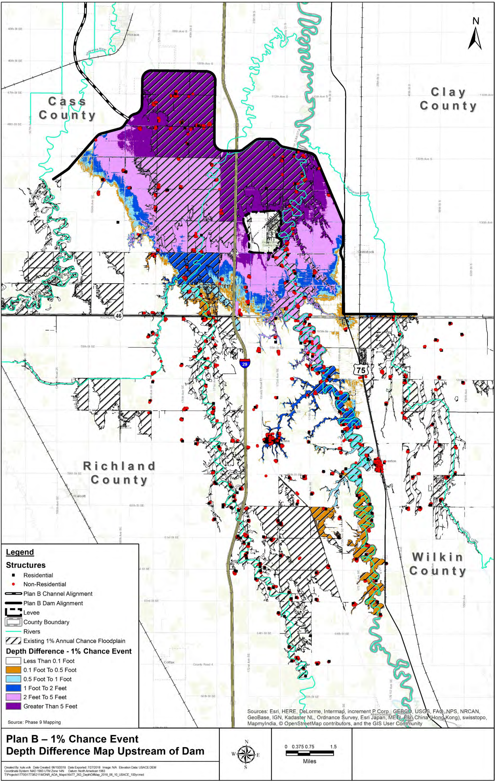
Figure 39: Depth Difference Pool, 1% ACE Event
