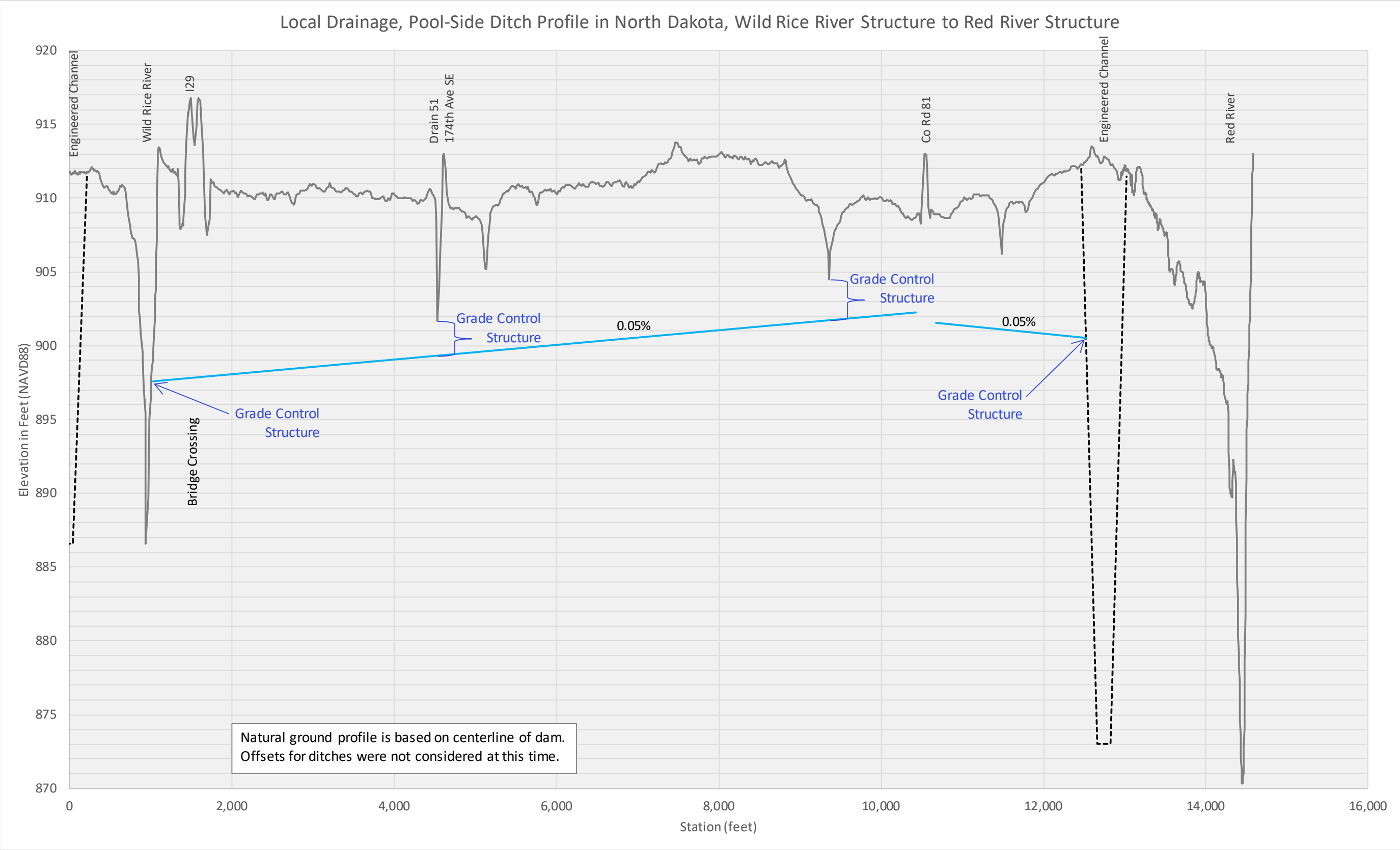
Figure 11. Pool-Side Ditch Profile in North Dakota, Wild Rice River Structure to Red River Structure
