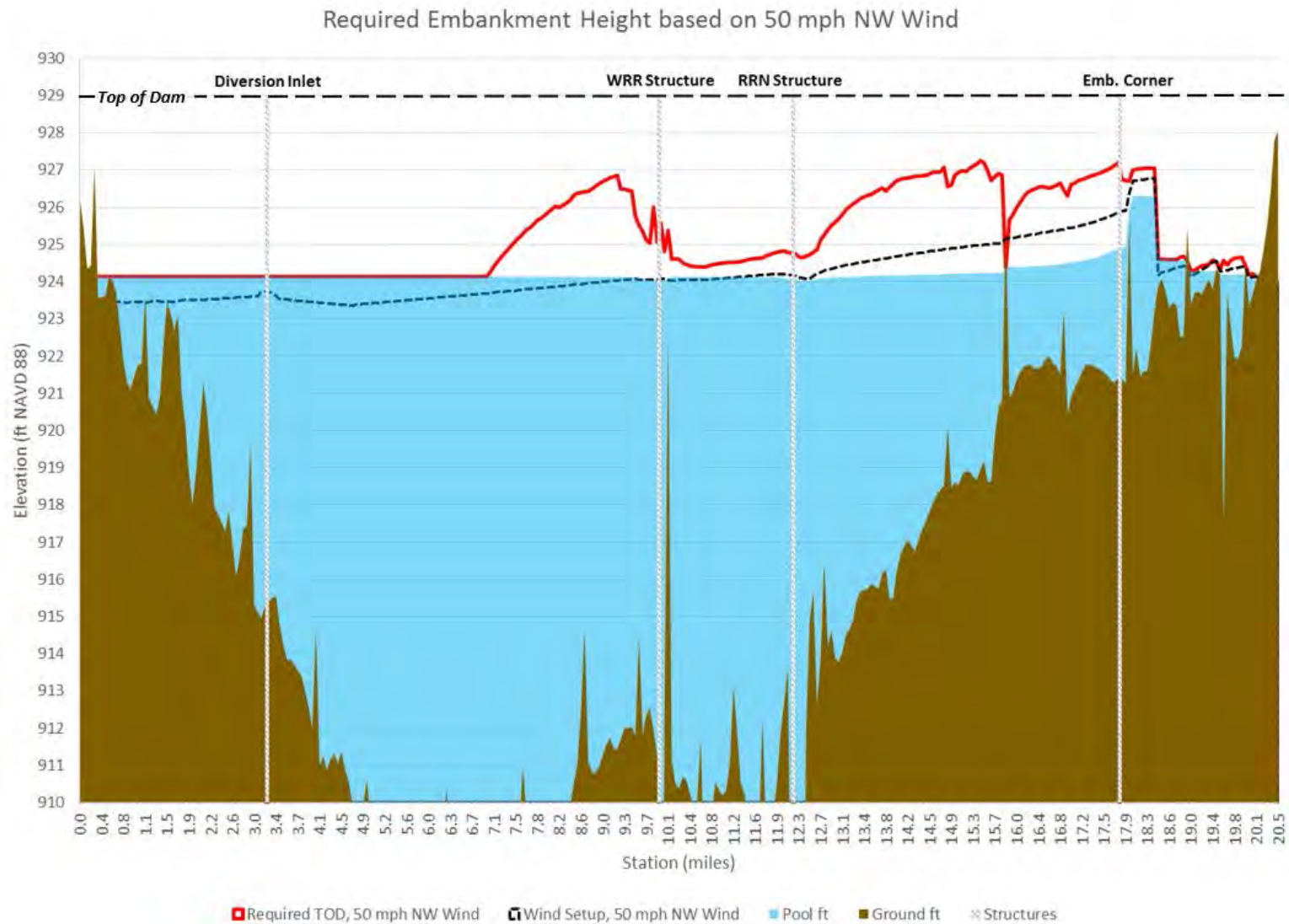
Figure 10: Required top of dam height for NW 50 mph wind conditions based on wave overtopping
