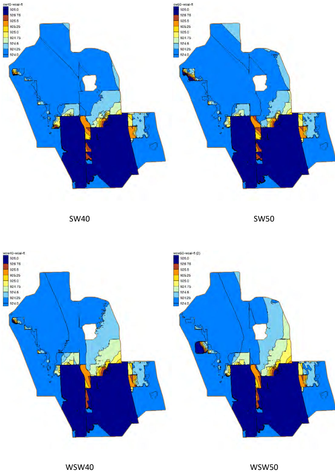
Figure 20: Water surface elevation with wind setup for winds from the southwest and west-southwest
